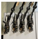
18180 Muller Martini HK 882 stitching head (4x) 4 stitching heads
