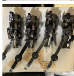
17905 Muller Martini HK 249 eyelet stitching head (4x) 4 eyelet stitching heads
