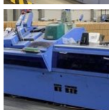
17547 Muller Martini 3696 gathering elements 2009 € 17.500.00 For extension of existing gatherer to Bolero/Alegro/Corona, with 1 base frame with 4 positions in total. 1 card gluer with Robatech Hotmelt system 1 standard feeder with 2 stations ASAC thickness control
